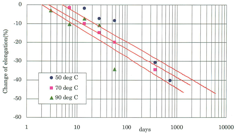
Fig.1) Relationship between change of elongation and days
