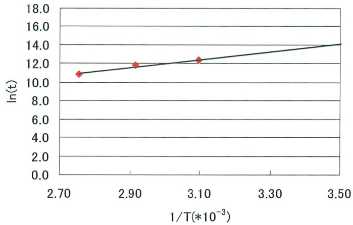
Fig.2 ) Relationship between ln (t) and (1/T)
